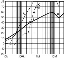
10A types
