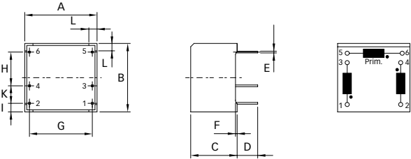
IT 242
