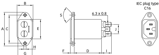
FN 9244E-HI
