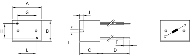
RI 415, RI 425
