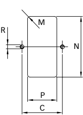
Panel cut out
