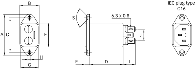
FN 9233-HI
