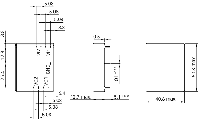
13A types
