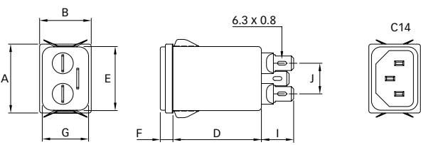
FN 9244S
