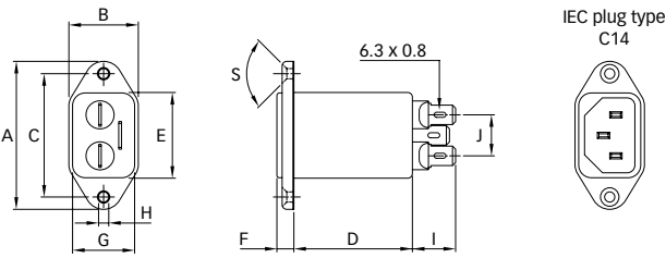
FN 9244
