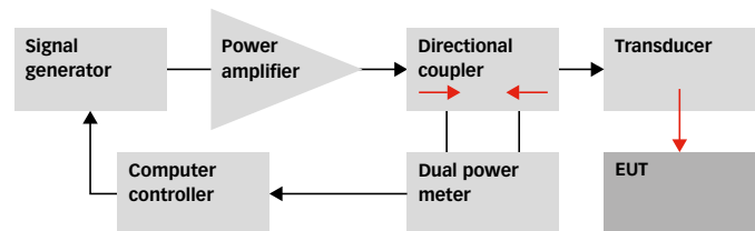
Testing principle for RF immunity
