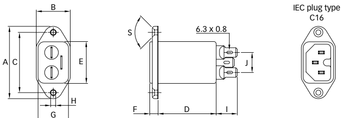
FN 9244-HI
