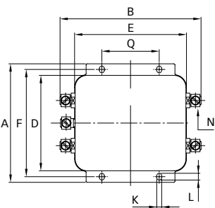
16A types
