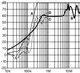
20A types
