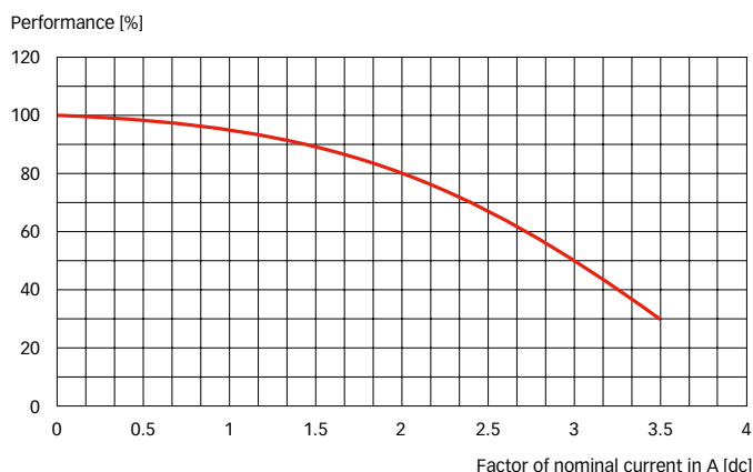
Saturation of chokes due to current
