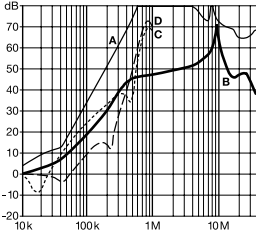
36A types
