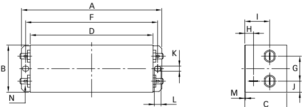
6A types
