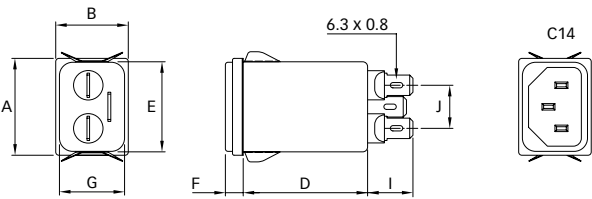
FN 9233U
