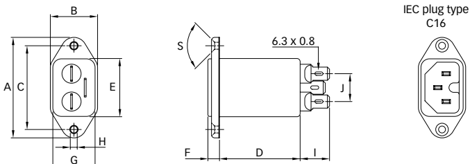
FN 9222E-HI
