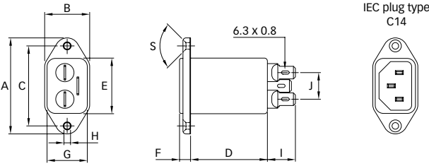
FN 9233
