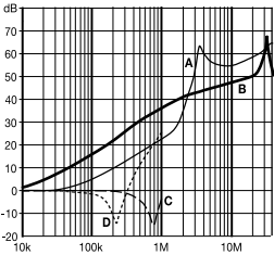
6A types
