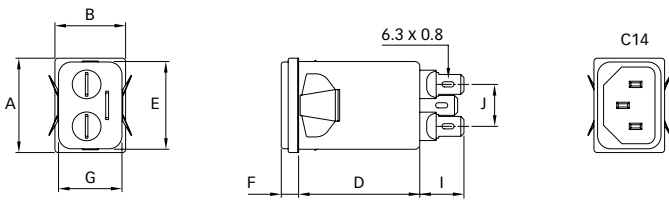
FN 9233ES1
