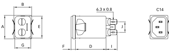
FN 9244S1
