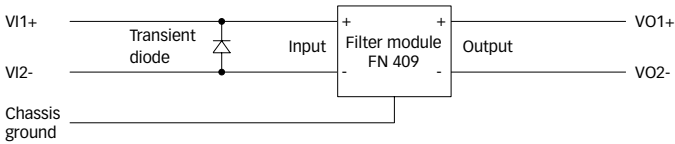
Figure 2: transient protection with a transient diode
