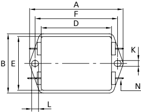
3A types
