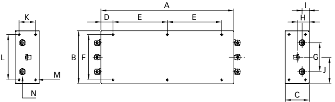
20A types
