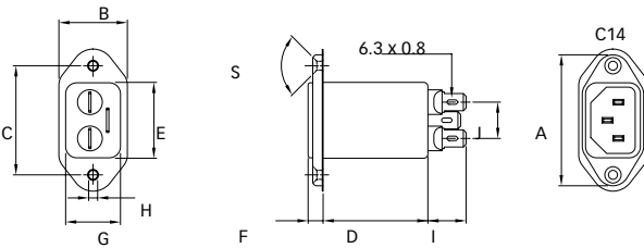
FN 9233U
