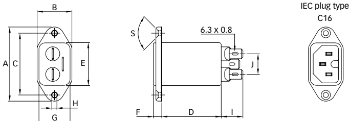
FN 9233E-HI
