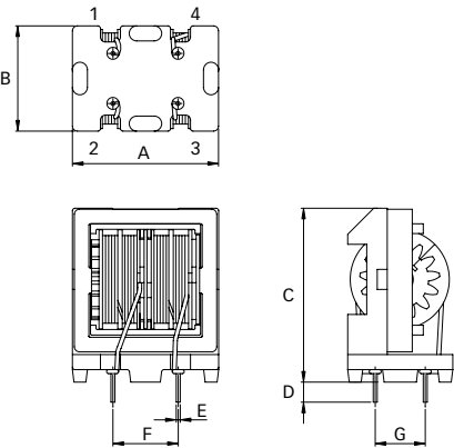
EH 20 to 35
