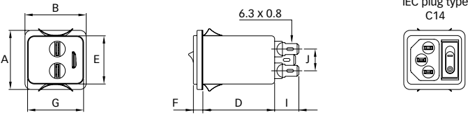
FN 9263S
