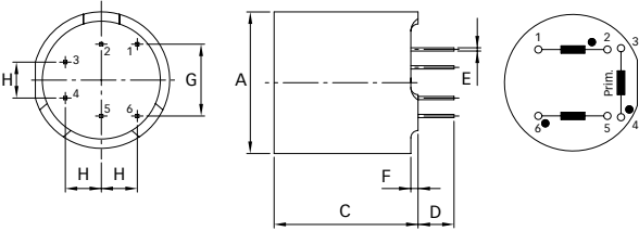
IT 213
